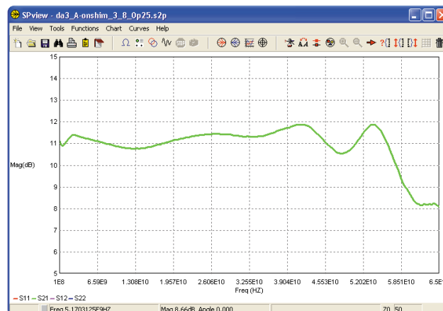
Broadband S-parameter data for DA3
