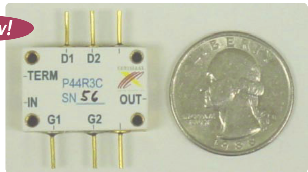
P44R3C EA Driver Amp (0.94 x 0.62 x 0.26 in)
